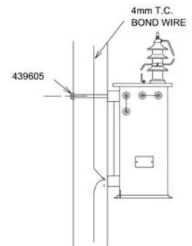
FIG. 2 POSITION OF SINGLE BOLT FIXING TRANSFORMER WHEN SPECIFIED
