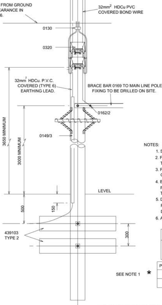
FIG. 2 POSITION OF SINGLE BOLT FIXING TRANSFORMER WHEN SPECIFIED
